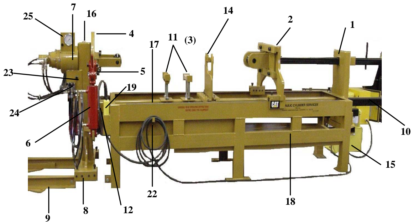
FIGURE 1. HCS-30 HYDRAULIC CYLINDER SERVICER
